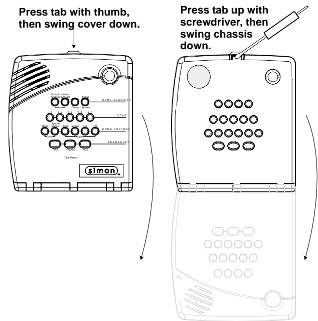
Figure 2. Opening the Panel Cover and Chassis
